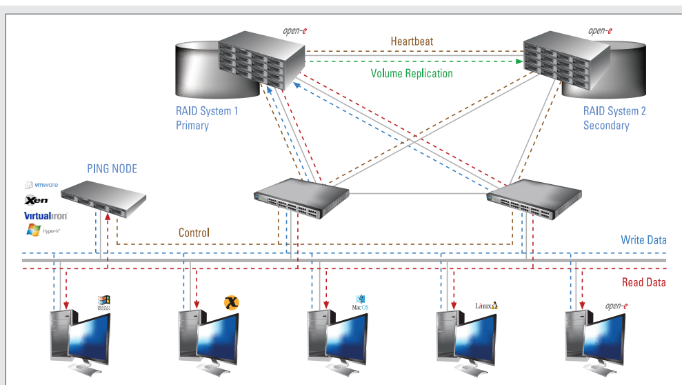
Figure 1 Open-E DSS with Automatic Failover
