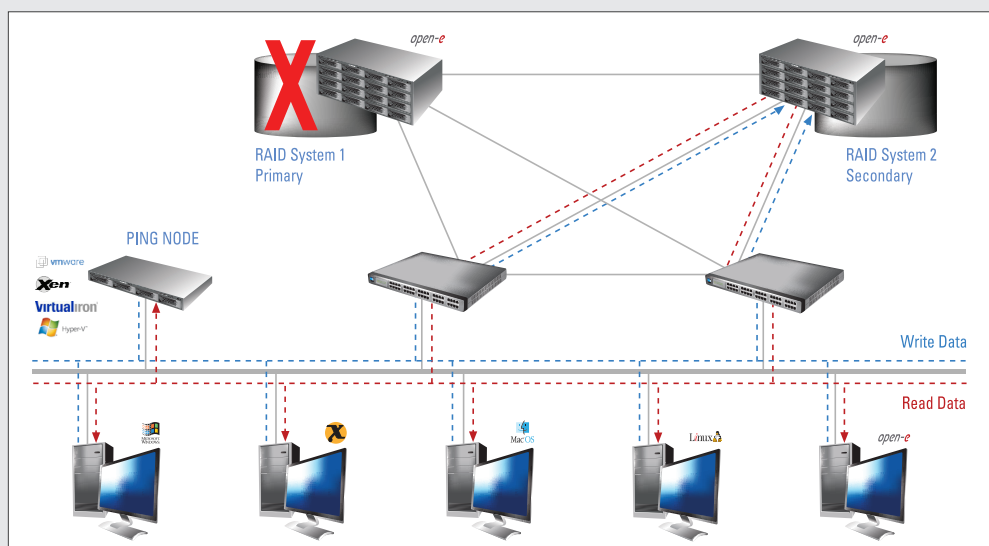
Figure 3 Open-E DSS Automatic Failover completed
